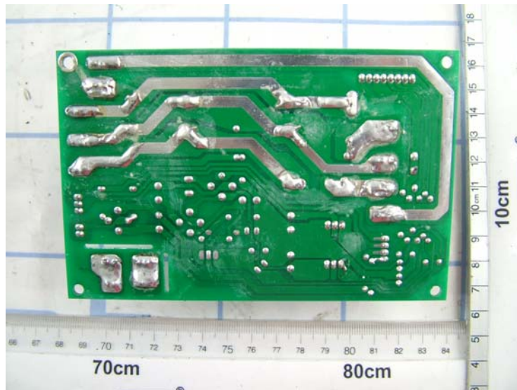
Figure 13 (PCB - solder side)
