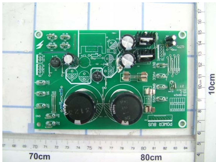
Figure 12 ( PCB - components side )
